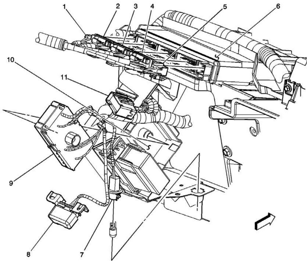
Fig. 16: Data Link Connector and Splice Pack SP205 Component View Courtesy of GENERAL MOTORS CORP.
